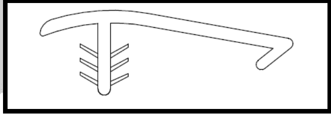
Die 1134 — 2-Part Vinyl To Tile Top
