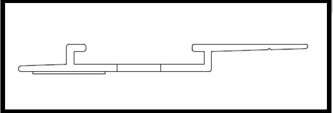
Die 1462 — Concealed Floor/Wall Trans Strip
