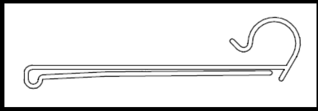
Die 1369 — 39mm Swing Ticket (For 8mm Wire)
