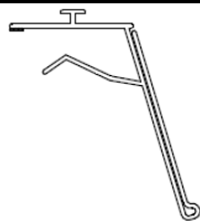
Die 1759 — 39mm Glass Adaptor with 'T'
