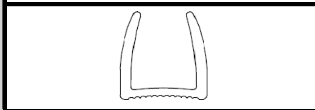
Die 1995 — 16mm Wide 'U' Channel
