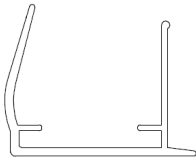
Die 1504 — 25mm End Closure
